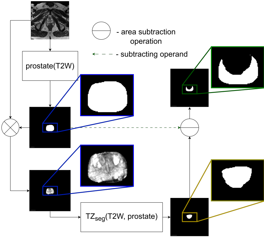
Figure 2.9. The prostate zone segmentation workflow: Prostate Segmentation, Transitional Zone Segmentation, and Peripheral Zone Calculation.
