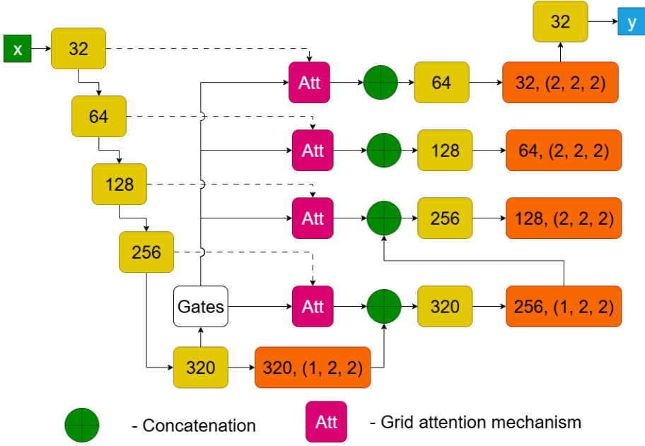
Figure 2.11. Diagram of the grid attention U-Net architecture
