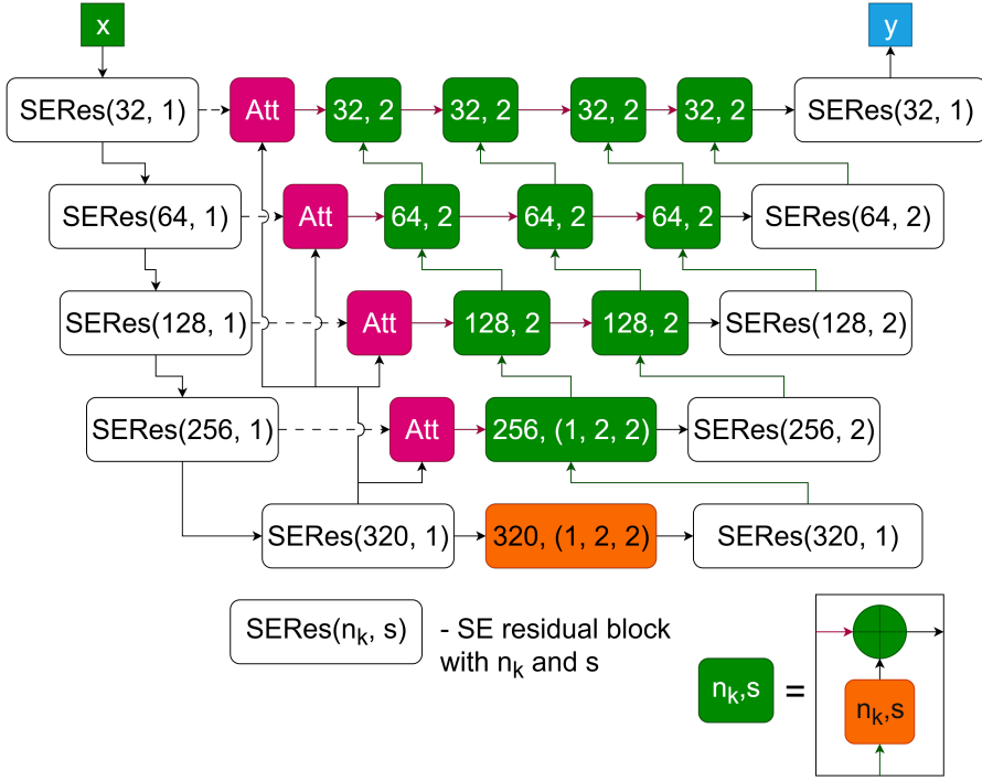
Figure 2.14. Diagram of the dual-attention U-Net
