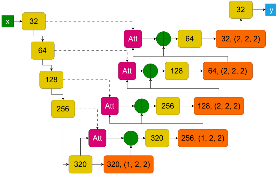
Figure 2.12. Diagram of the single attention U-Net architecture
