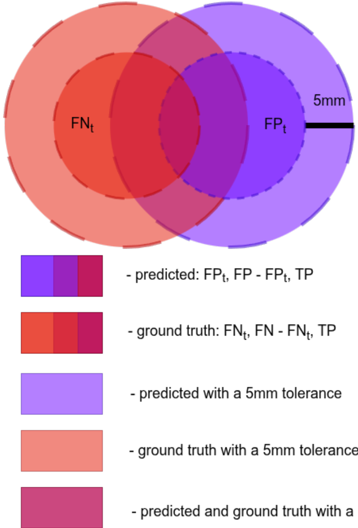
Figure 2.15. Venn diagrams illustrating the calculation of FN_\tau and FP_\tau .
