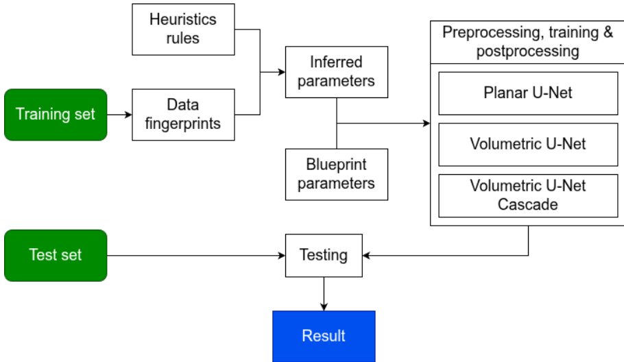
Figure 2.1. The workflow the of the no-new U-Net method.
