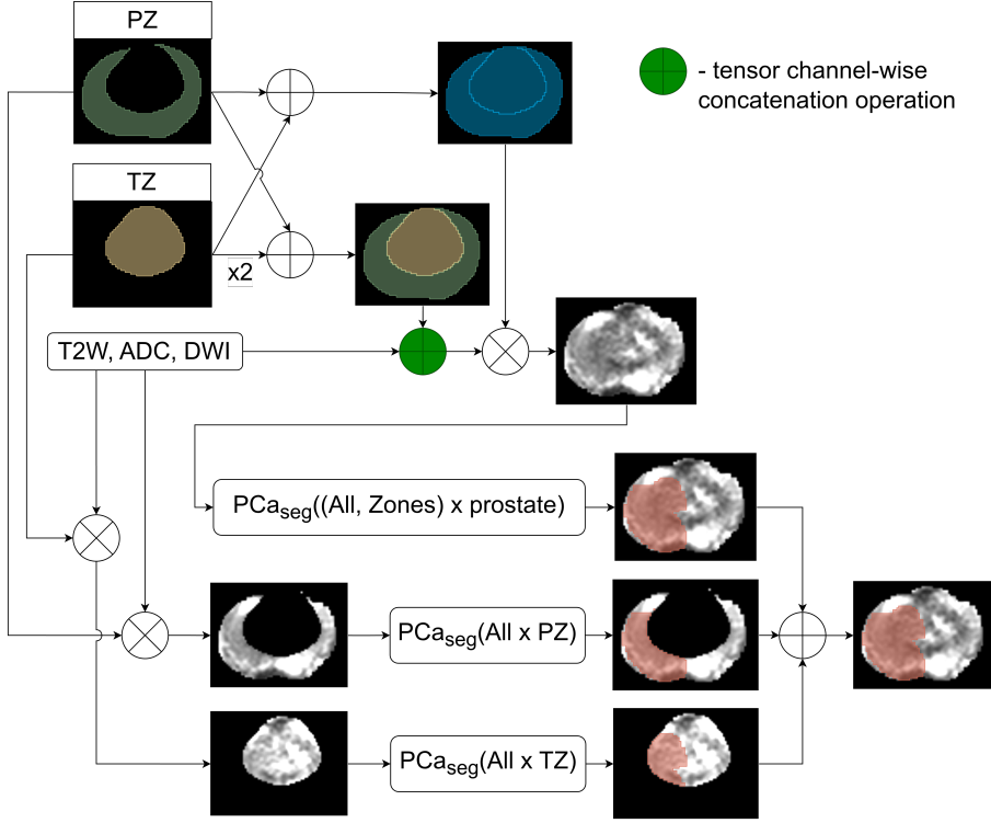
Figure 2.6. Ensemble 3 workflow diagram.
