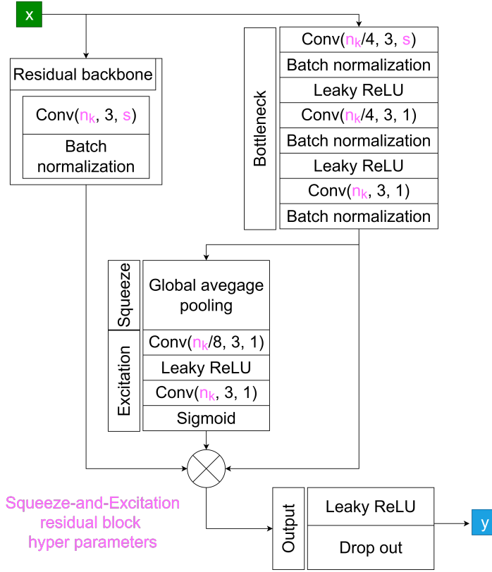
Figure 1.2. Schematics of the Squeeze-and-Excitation residual block.
