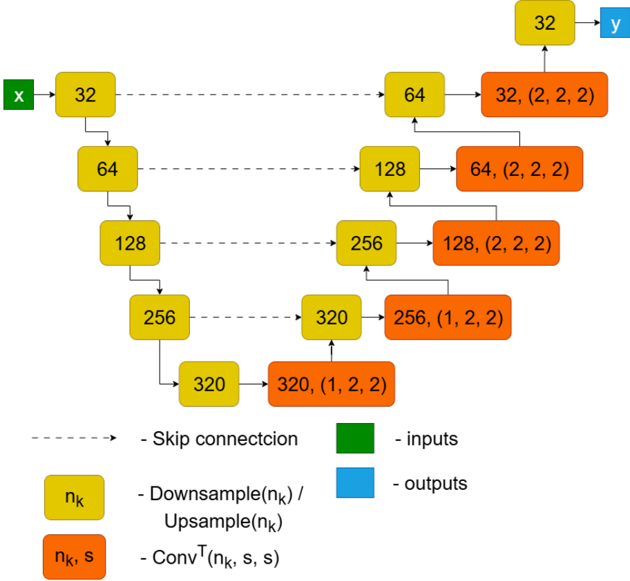
Figure 2.2. U-Net architecture with hyperparameters used in the no-new U-Net method.
