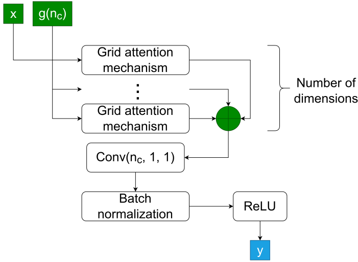
Figure 2.13. Diagram of the multidimensional attention mechanism
