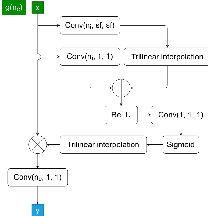
Figure 2.10. Diagram of the grid attention mechanism
