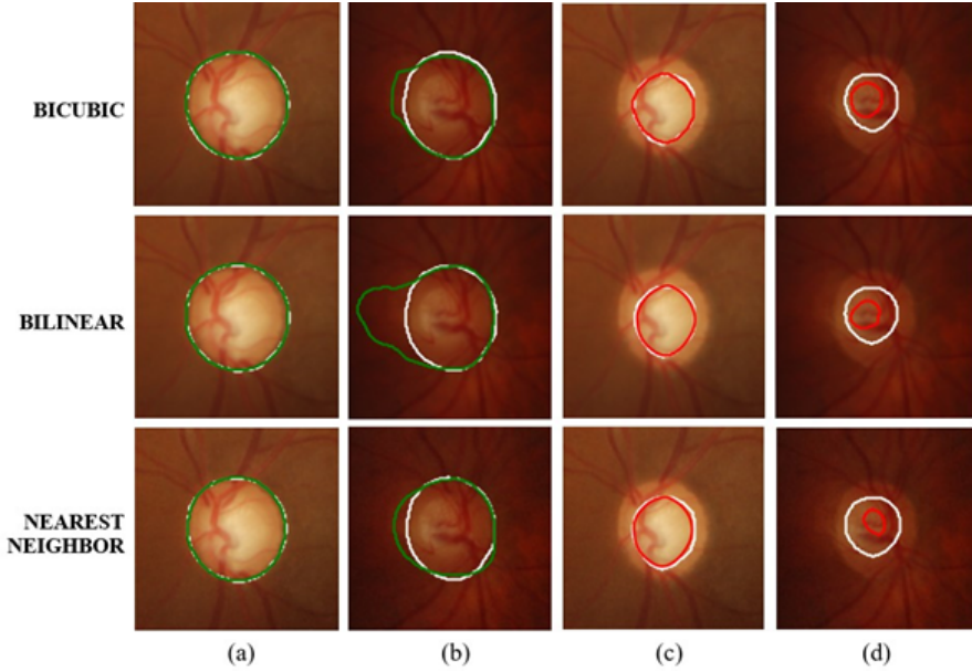
Figure 3.2: OD (green) and OC (red) segmentation results using different interpolation methods with Attention U-Net. (a) Best-case OD segmentation, (b) Worst-case OD segmentation, (c) Best-case OC segmentation, (d) Worst-case OC segmentation. The white circle indicates the ground truth.
