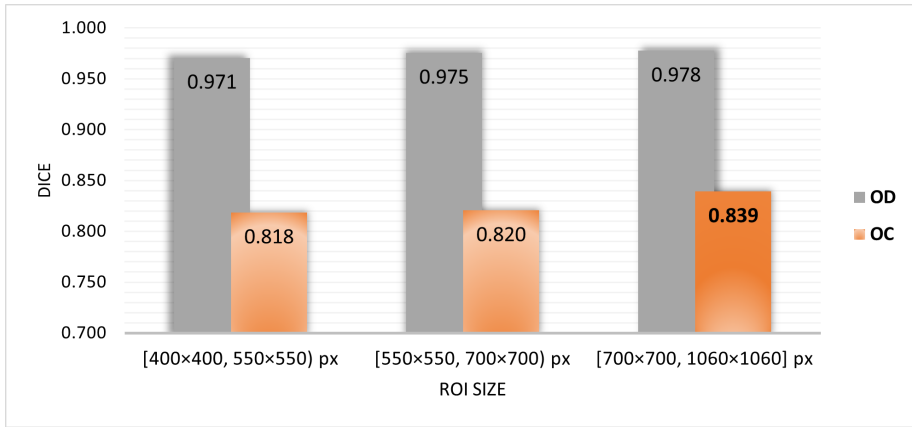
Figure 3.1: Distribution of Dice for OD and OC segmentation on images resized via bicubic interpolation from the initial ROI to 512×512 px.
