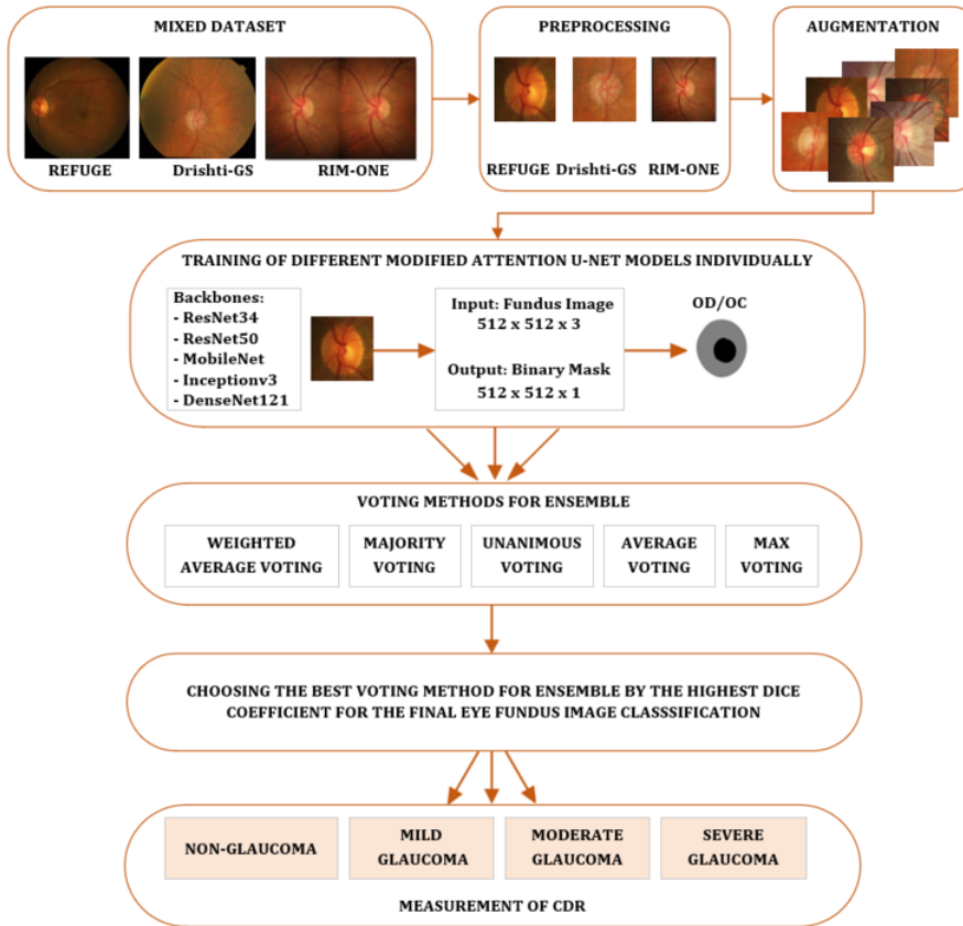
Figure 3.3: Flowchart of the proposed DL ensemble method.
