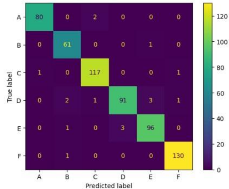
(b) fastvit_ma36
