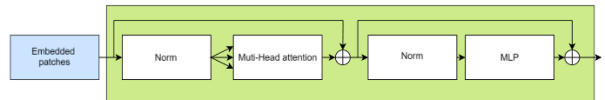
Figure 4: Transformer Encoder.
