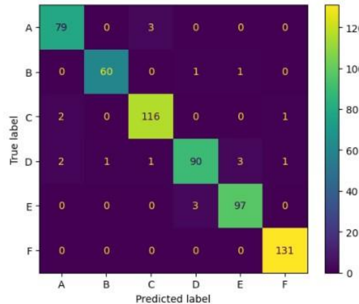
(a) resnet50
