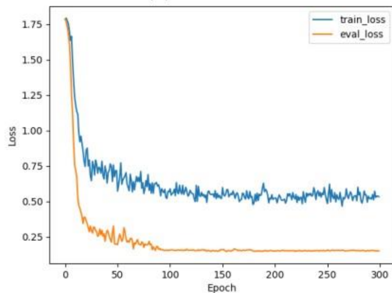
(c) convmixer_1536_20
