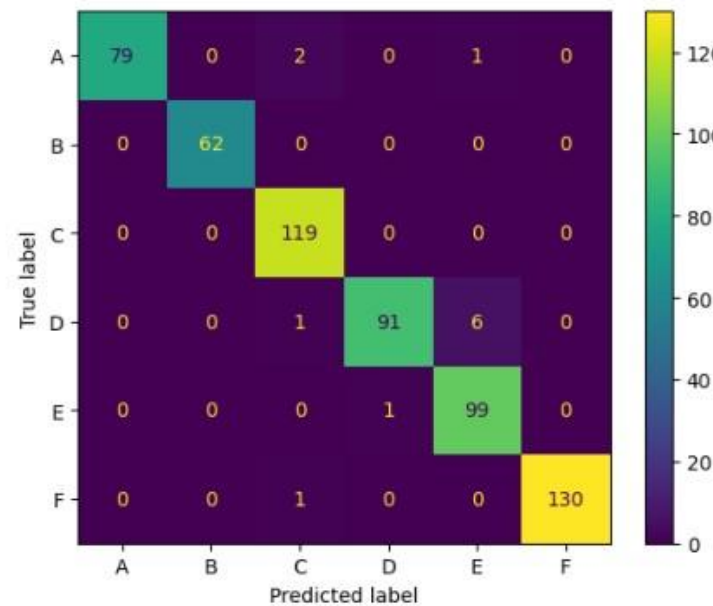
(c) convmixer_1536_20
