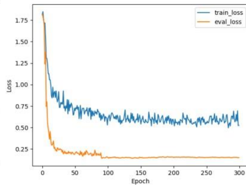
(b) fastvit_ma36
