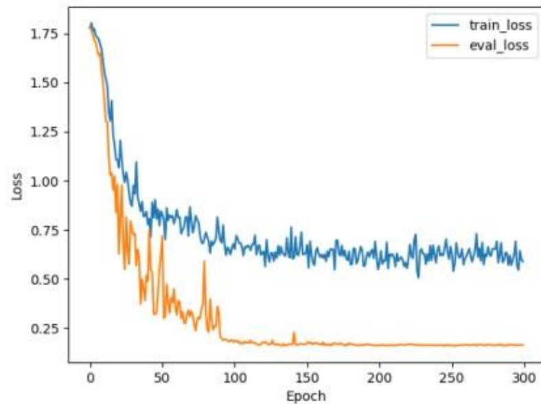
(a) resnet50
