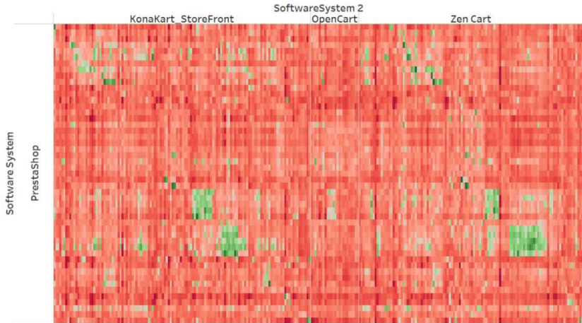
Fig. 6. Operation interoperability scoring – a heatmap using the average ensemble score of edit distance algorithms; the green spots indicate above 50% similarities.
