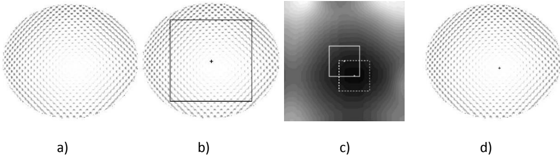
Figure 16. Lateral chromatic aberration focus center detection in G-R
