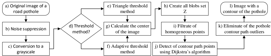
Figure 3. Contour recognition scheme for pothole detection.
